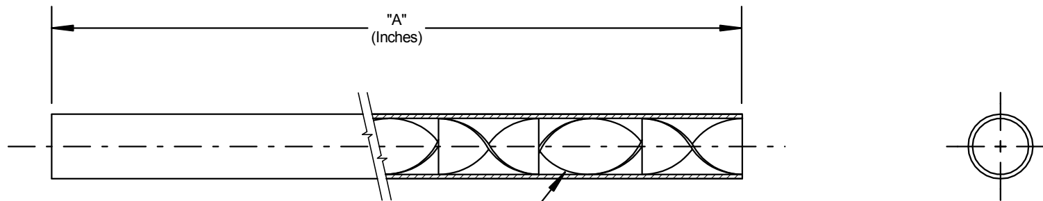
KOFLO STRATOS HIGH PRESSURE TUBE MIXER WITH * _____ HELICAL MIXING ELEMENTS
